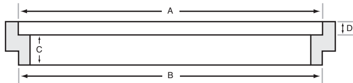
SECTION X-X
